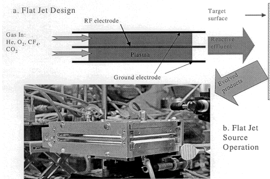
Fig. 5: Schematic drawing (a) of the flat jet and a photograph of the same in operation (b).
