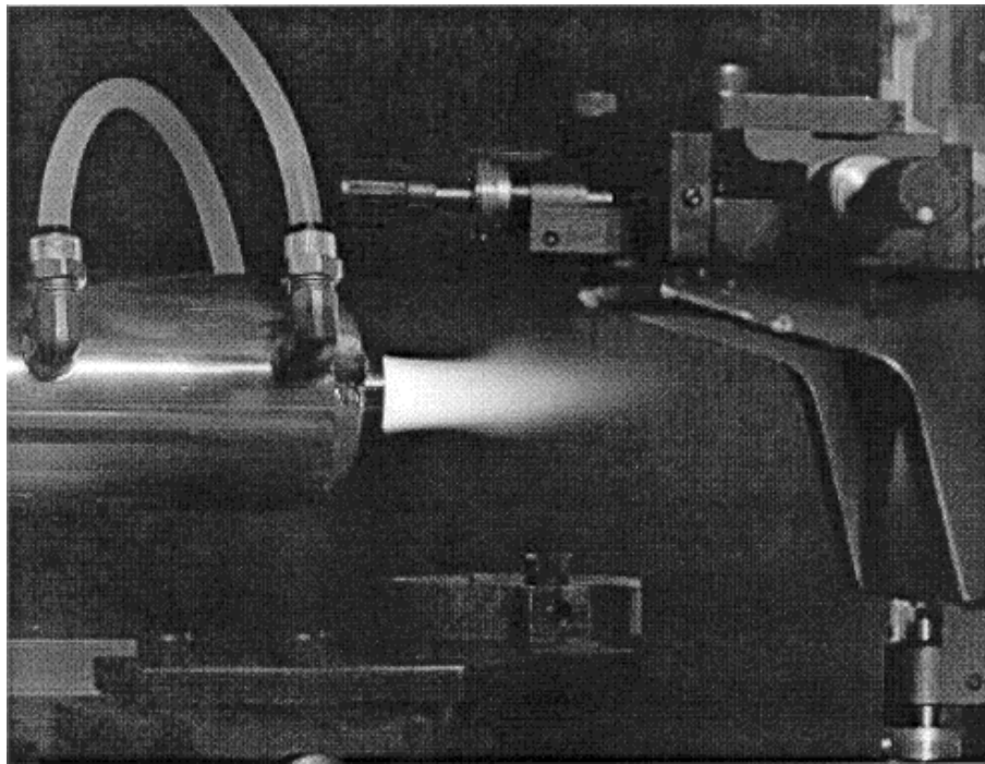
Fig. 4: Operation of a cylindrical version of the atmospheric pressure plasma jet. Note the effluent stream of reactive chemical species that exits from the end of the APPJ source.
