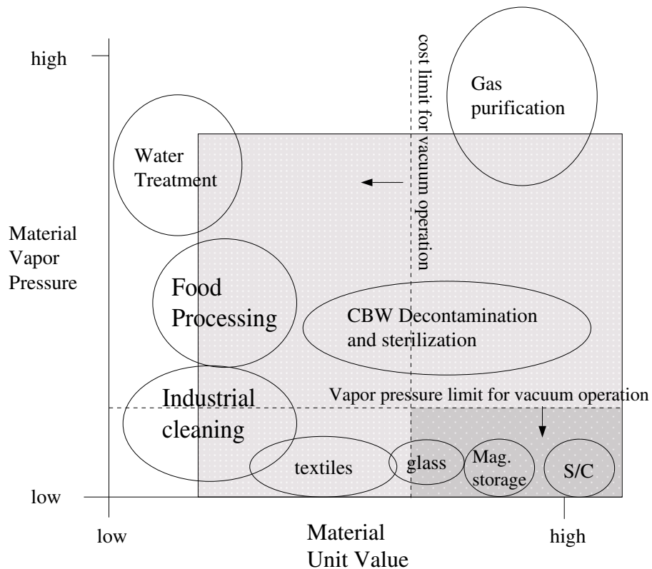
Fig. 1: Comparison of the process limits resulting from vapor pressure and economic constraints for both vacuum and atmospheric pressure plasma processing. The rectangular box in the lower right corner represents the domain for vacuum processing. The larger box represents the domain constraints for atmospheric pressure plasma processing. The larger box also contains much of the process domain represented for vacuum-based plasma processing.
