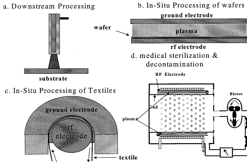
Fig. 6: Variations in use of the APPJ technology and different source designs.
