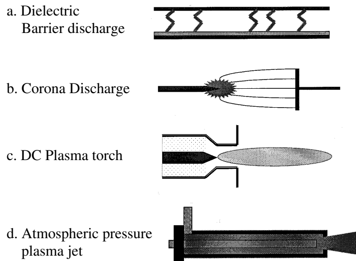
Fig. 3: Four different kinds of atmospheric pressure plasma sources.
